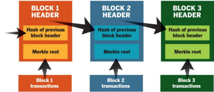
SIMPLIFIED BITCOIN BLOCK CHAIN
